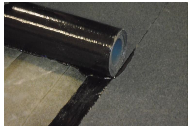
Figure 2 Side Lap Formation
