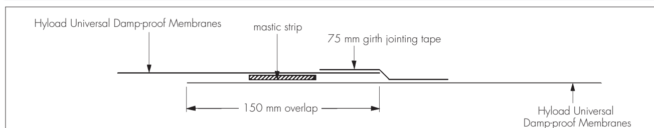
Figure 1 Mastic tape joint
