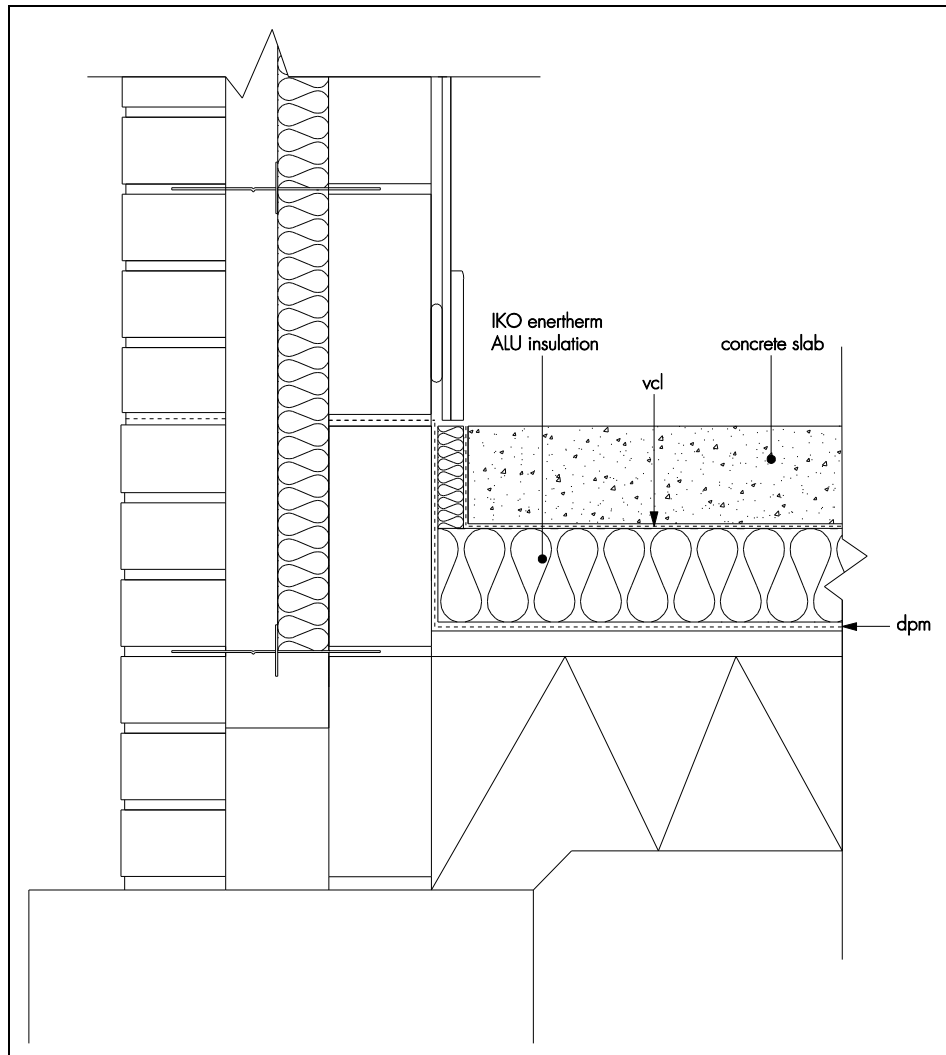
Figure 2 Ground-supported concrete floor — concrete slab overlay
