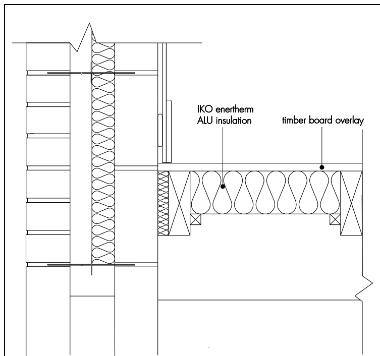
Figure 4 Suspended timber floor — board overlay
