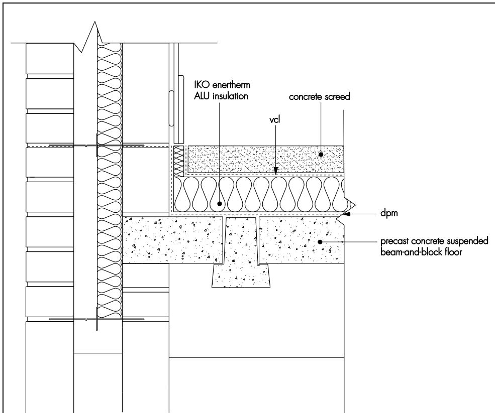
Figure 3 Suspended concrete beam-and-block floor — screed overlay
