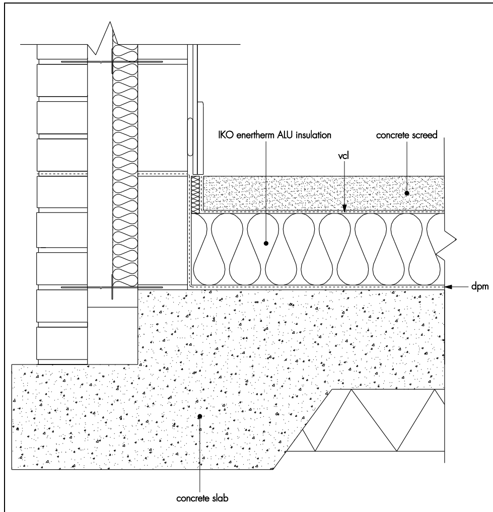
Figure 1 Ground-supported concrete floor — screed overlay
