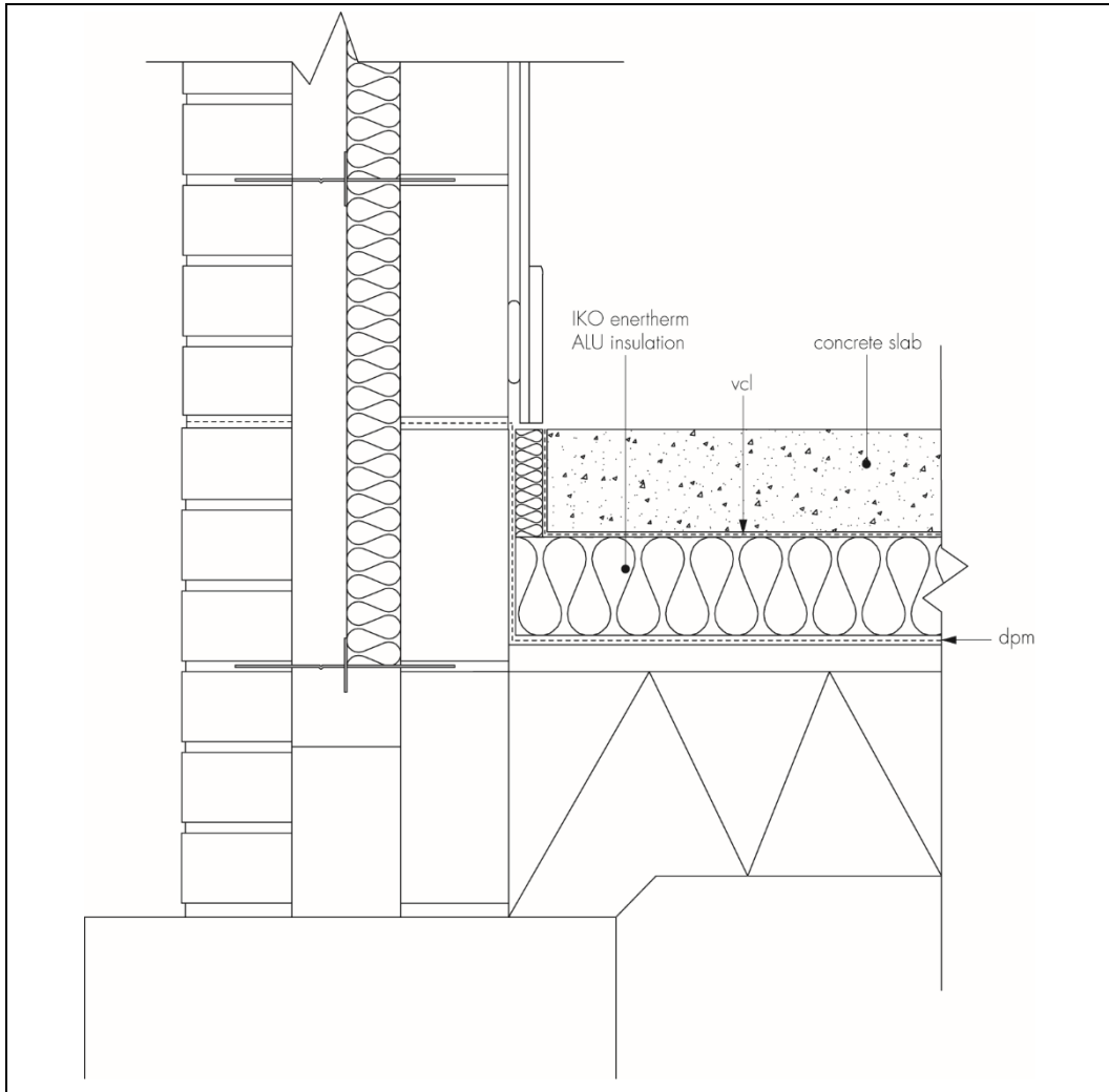
Figure 2 Ground-bearing concrete floor – concrete slab overlay
