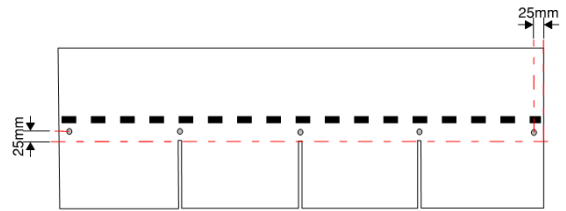
Figure 2 - Installing the shingle
