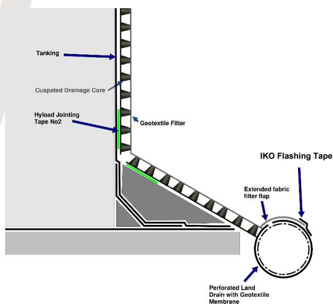
Figure 2 - Interface with perforated land drain
