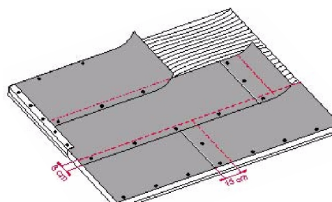
Figure 1 - Installing the underlay
