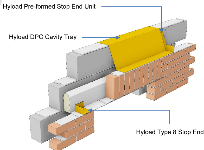
Figure 5 – Typical Hyload Cavity Tray above lintel position
