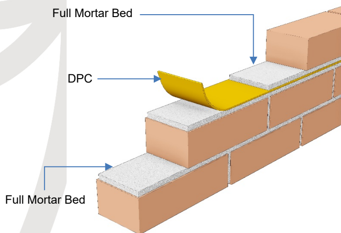
Figure 3 – IKO Hyload DPC bedding
