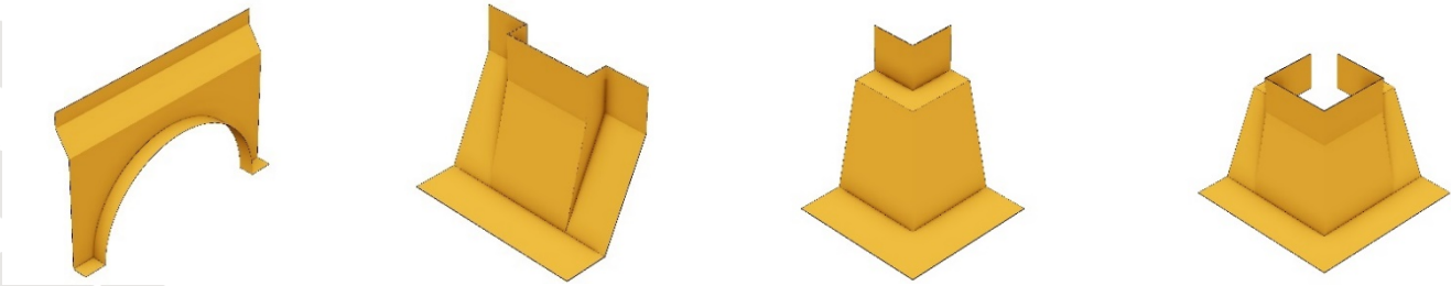
Figure 2 – Example selection of bespoke Hyload Pre-formed Cloak Units
