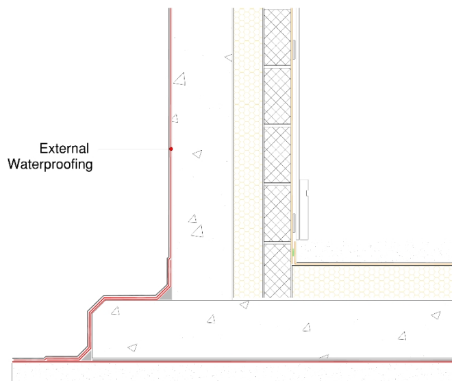
Figure 1 – Typical External Membrane Application
